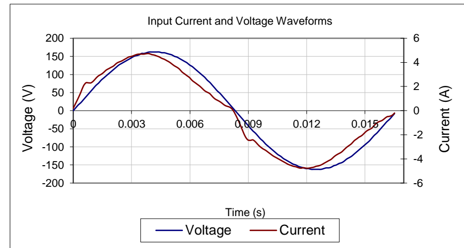
Input AC Current Waveform (ITHD = 7.46%, 50% Load)
